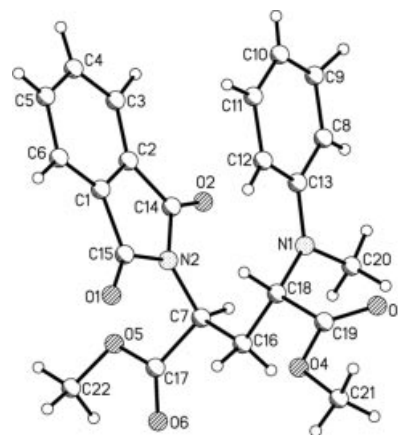
Figure 1. X-ray structure of glutamic acid derivative (2 S ,4 S )- 2 .
