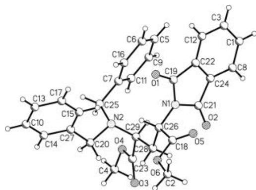
Figure 2. X-ray structure of glutamic acid derivative threo - 4 .
