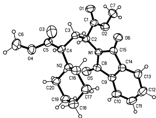
Figure 3. X-ray structure of glutamic acid derivative erythro-5 .
